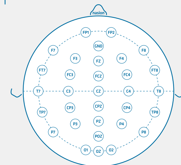
32 Electrodes Scheme
